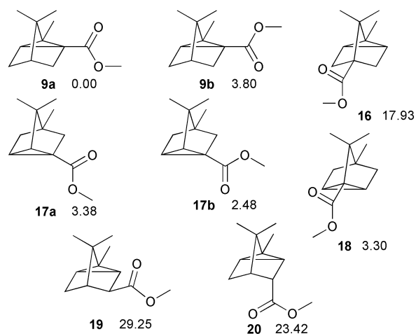
Fig. 1 Relative energies in \text{kJ mol}^{-1} of isomeric tricyclic esters \text{C}_{12}\text{H}_{18}\text{O}_2 .
