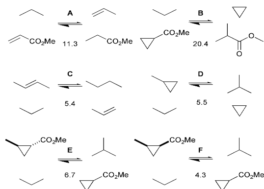
Fig. 2 Isodesmic reactions; energies in \text{kJ mol}^{-1} .
